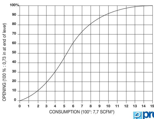
Pneumatic flow rate at 87 PSI for 27202 PRE
