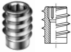
RAMPA Inserts type SK
